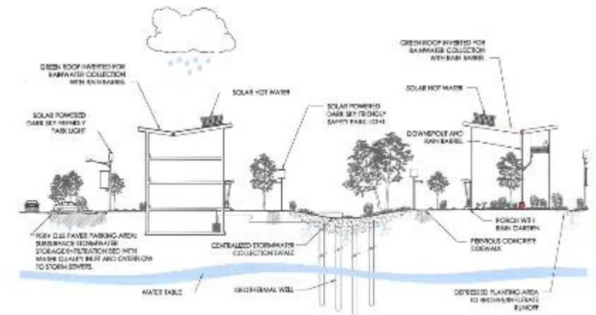
Central Park: Section
